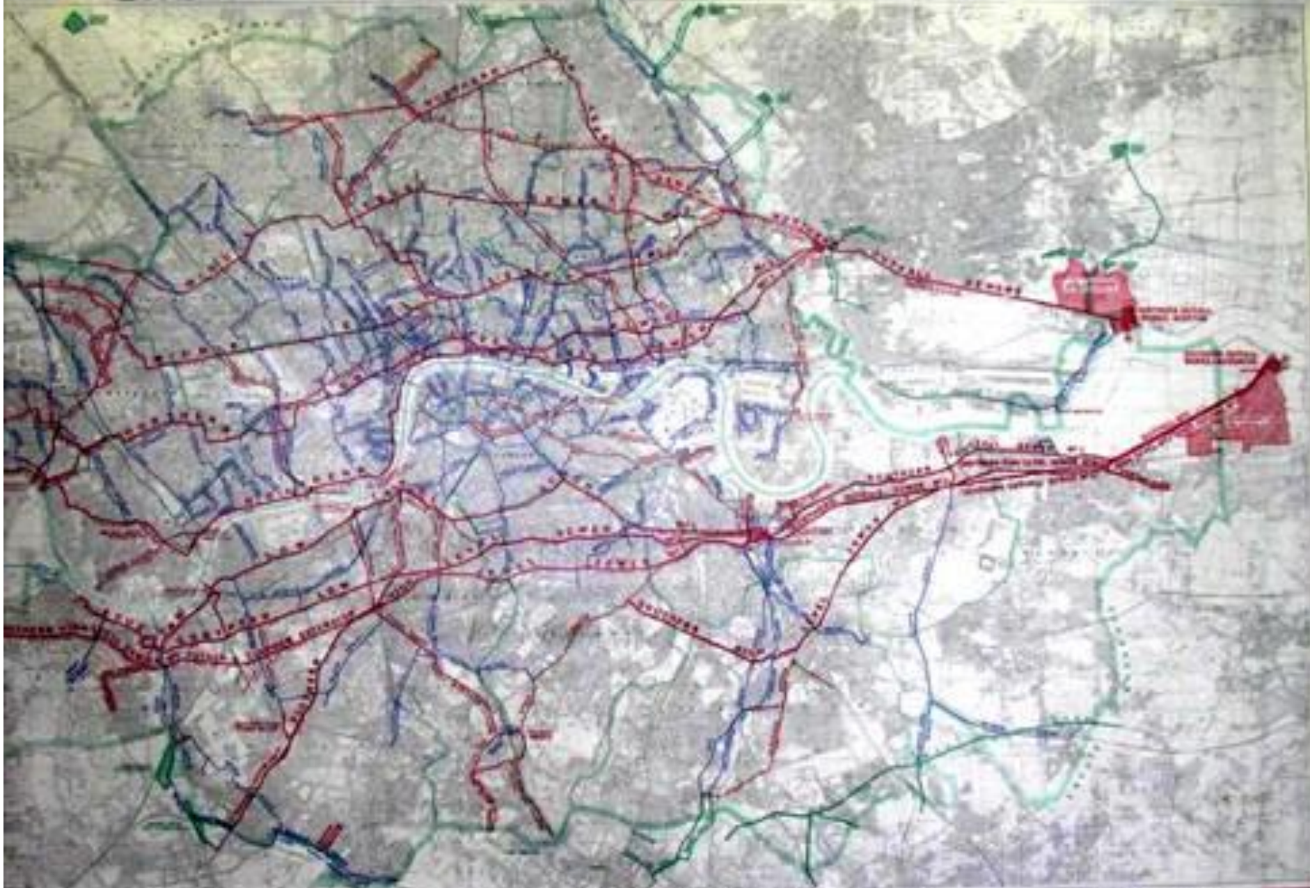
MAP SHOWING MAIN, INTERCEPTING AND STORM RELIEF SEWERS
